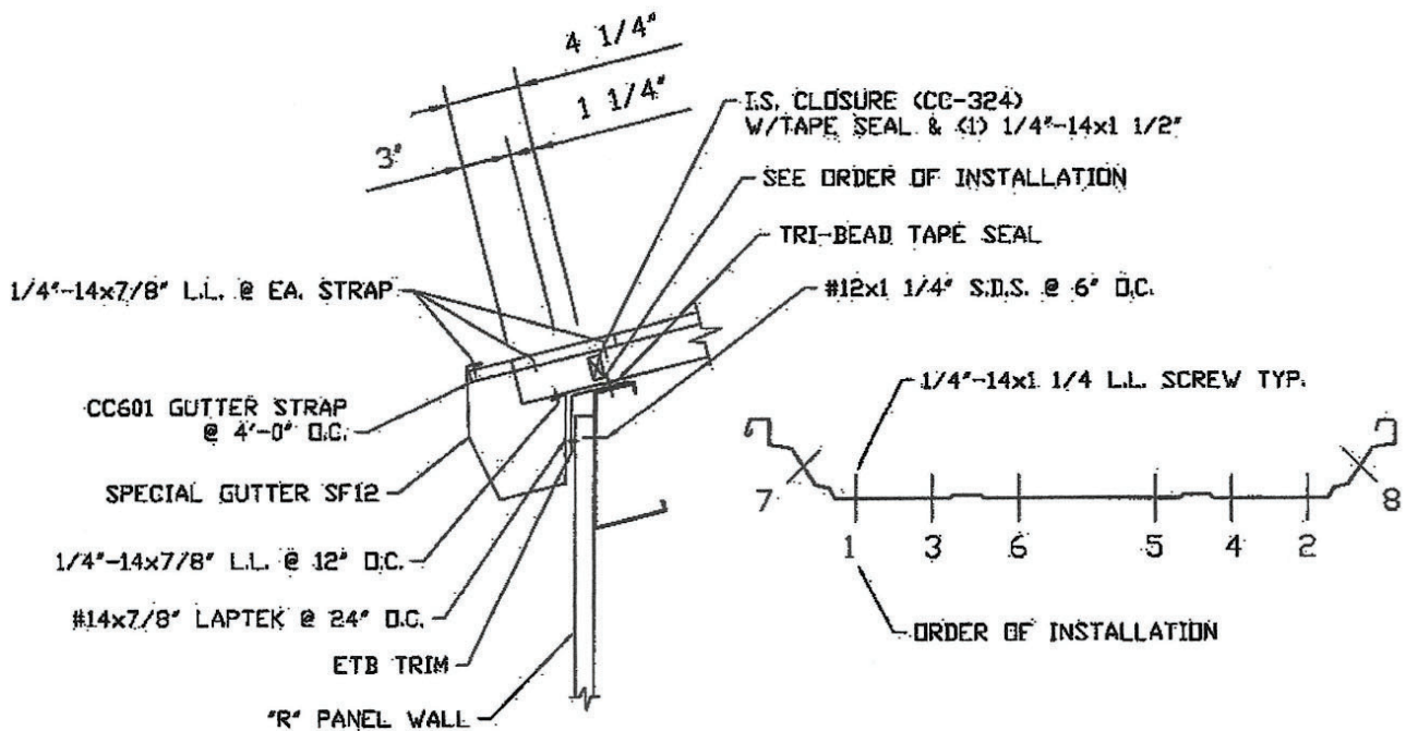
GUTTER DETAIL
